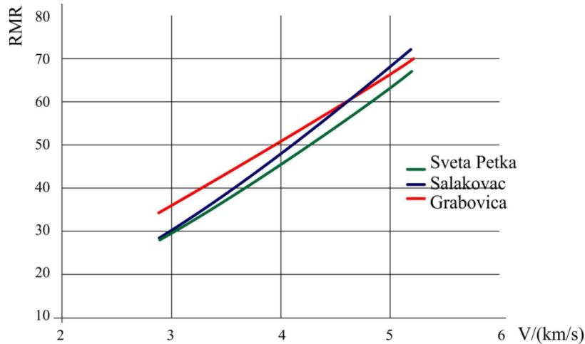
Figure 4. Regression curves between quality of rock mass RMR and velocities of longitudinal elastic waves v_1 from the location on „Salakovac“ dam RMR=9.8519 x v_1^{1.1721} and „Grabovica“ dam
