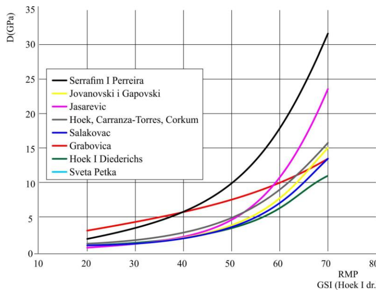
Figure 5. Correlative dependences between quality of rock mass RMR (GSI) and deformation modulus D from the location on „Salakovac“ dam D=0.1369 x e^{0.065RMR} (GPa), „Grabovica“ dam D=1.6963 x e^{0.0295RMR} (GPa), and „Sveta Petka“ D=0.1104 x e^{0.0703RMR} dam with known correlative dependences from literature [2, 5]
