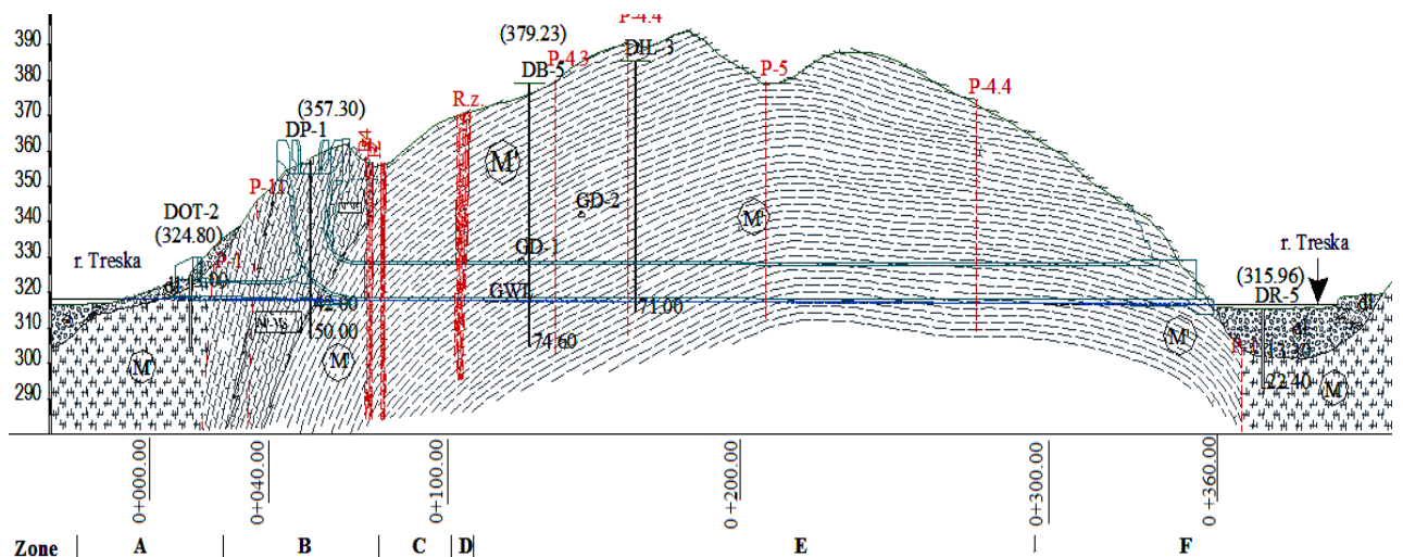
Figure 2. Engineering Geological Section for hydro technical tunnel for arch dam "Sveta Petka" in Republic of Macedonia
